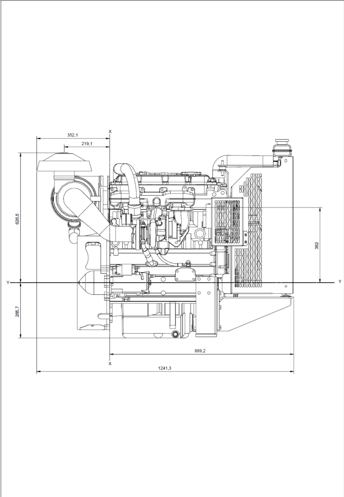
1104A-44TG2 ElectropaK - right view
