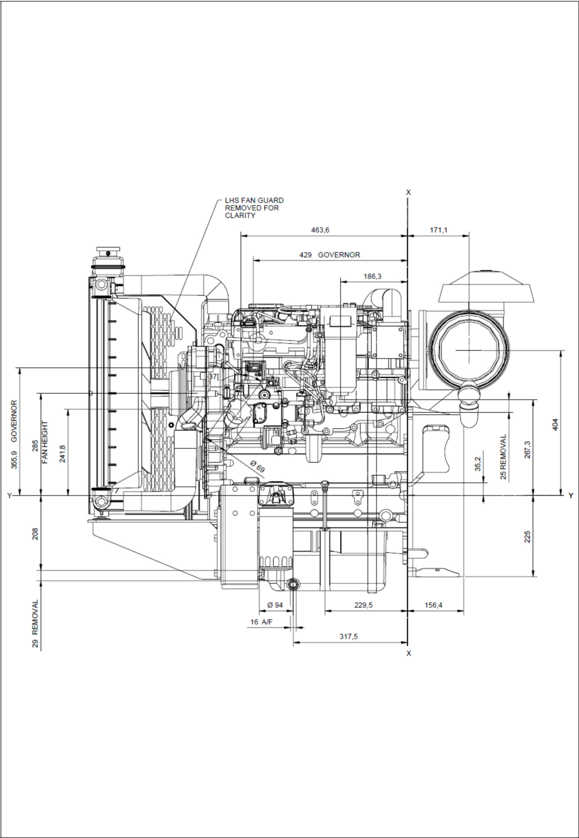
1104A-44TG2 Electropak - left view
